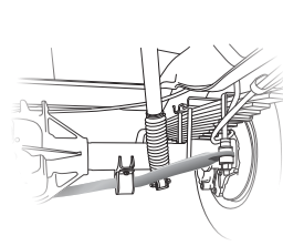
STANDARD FRONT & REAR STABILIZER BARS Reduces the body roll of a vehicle during fast cornering or over road irregularities
