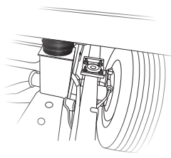
RUBBER ISOLATION MOUNTS Positioned near the tires to absorb road shock, dampen noise and minimize vibrations
